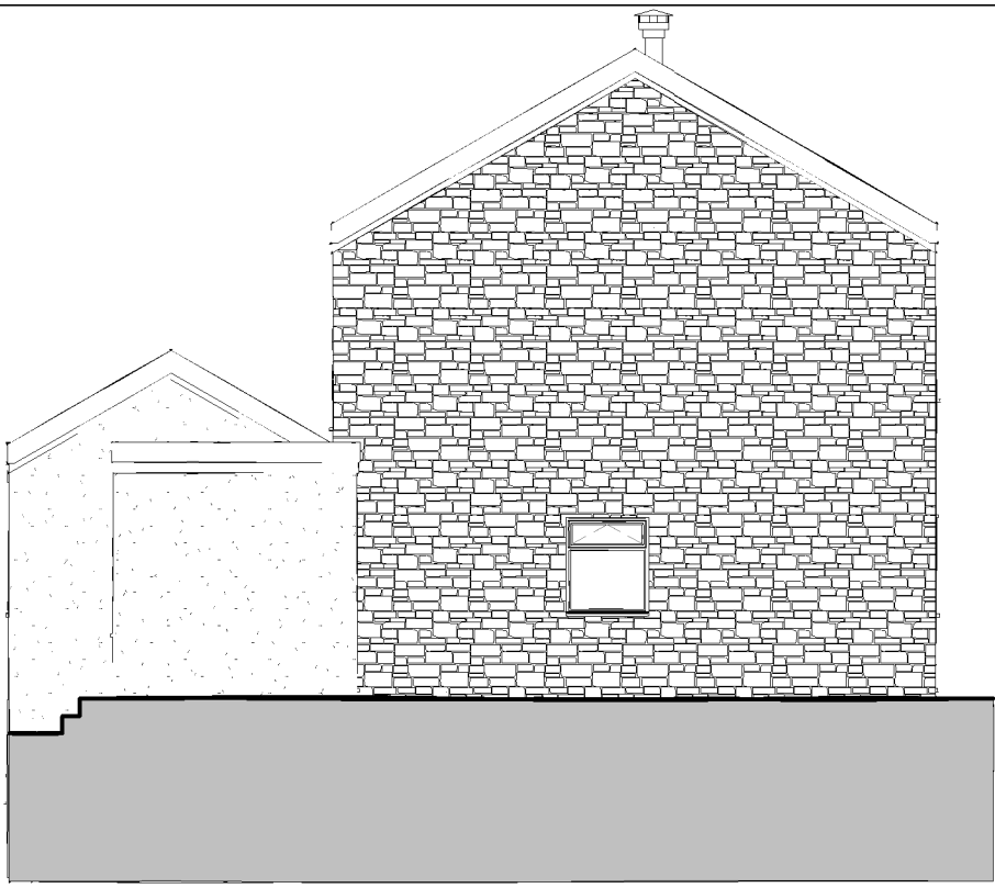
Existing Left Elevation
