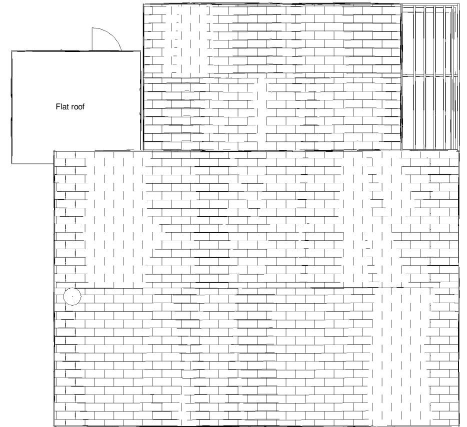
Existing Roof 1 : 100
