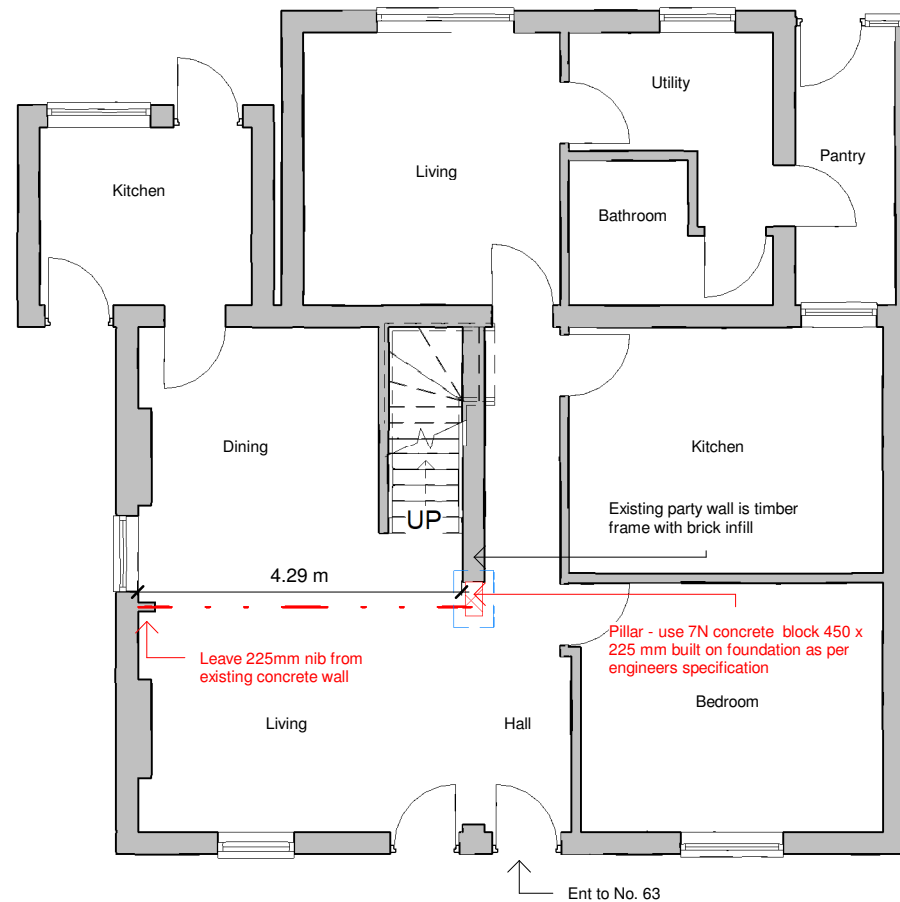
Proposed GF 1 : 100
