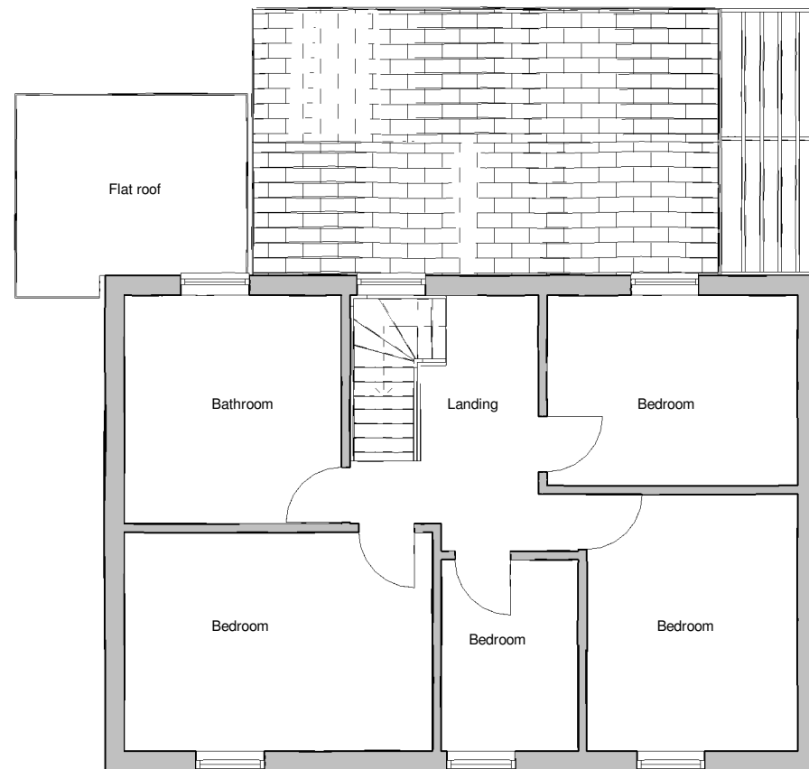
Proposed FF 1 : 100
