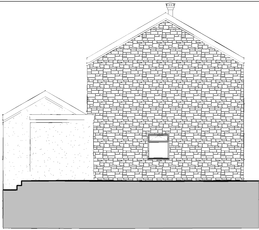
Proposed Left Elevation
