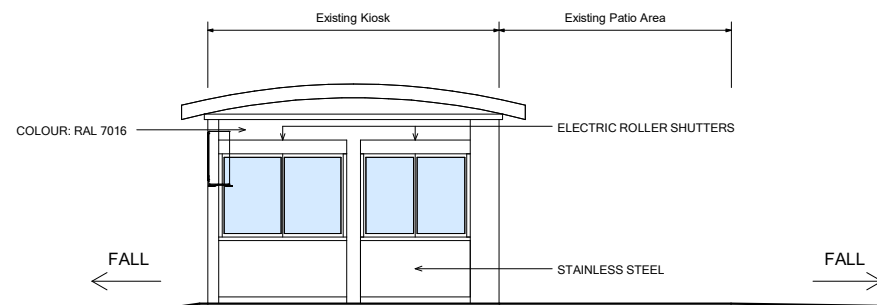
Existing West Elevation 1 : 50
