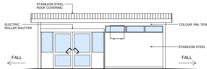
Existing South Elevation 1 : 50
