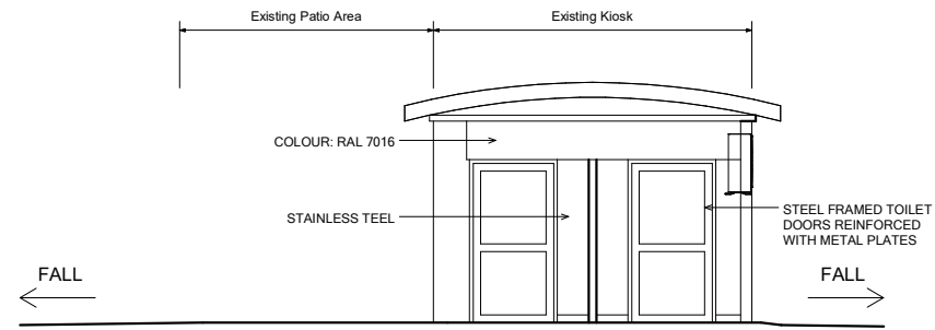
Existing East Elevation 1 : 50
