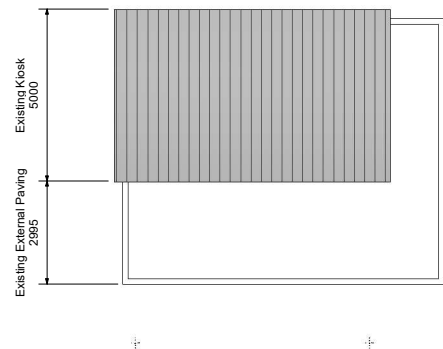
Existing Roof Plan 1 : 100
