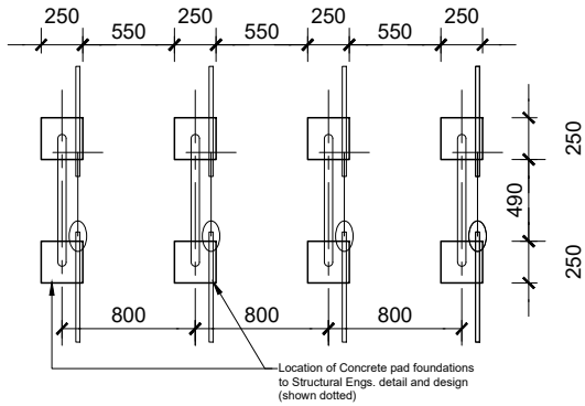
TYPE 4 - 4 No. Retail Bike Stand Plan
