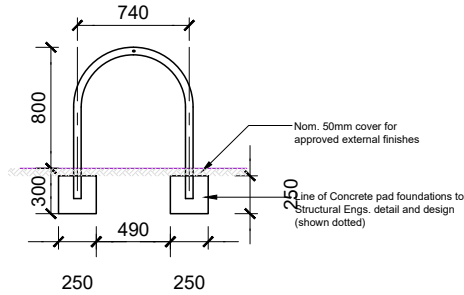
Typical Cycle Stand Bracket 4 No.
