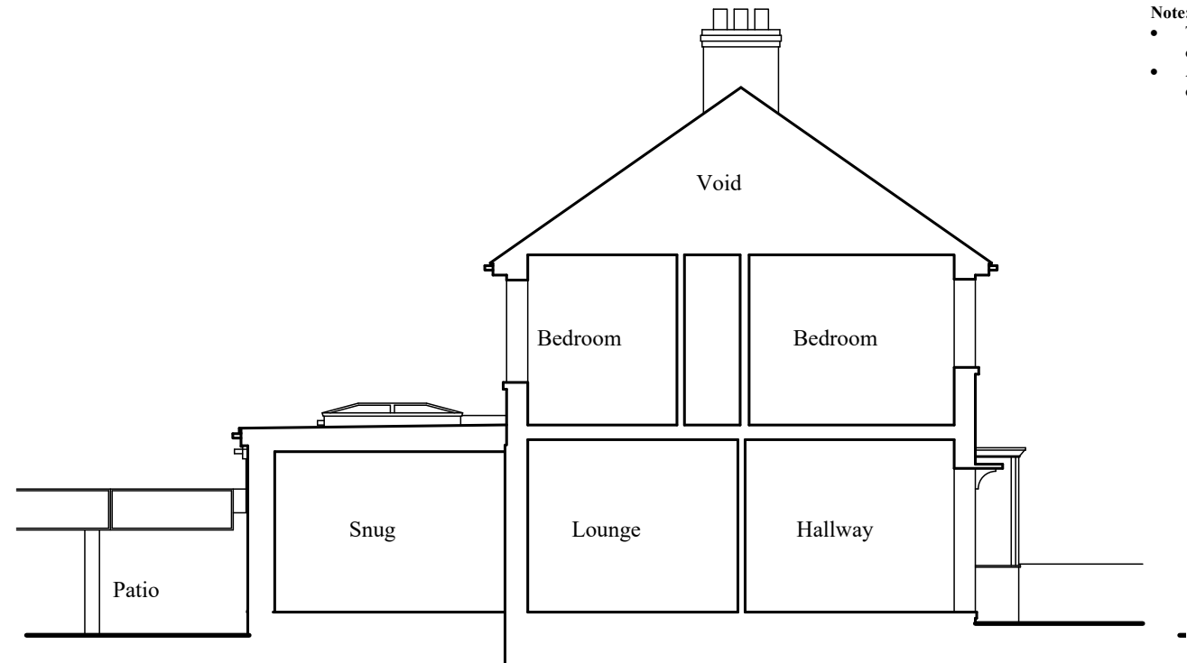
Section A
