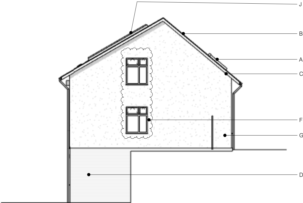
Side Elevation
