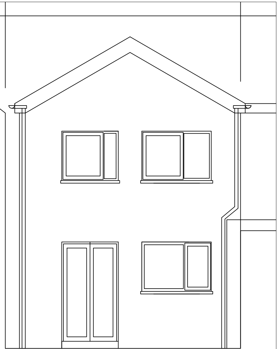
PROPOSED REAR ELEV
