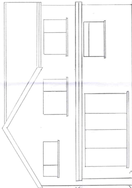
REAR ELEVATION PROPOSED
