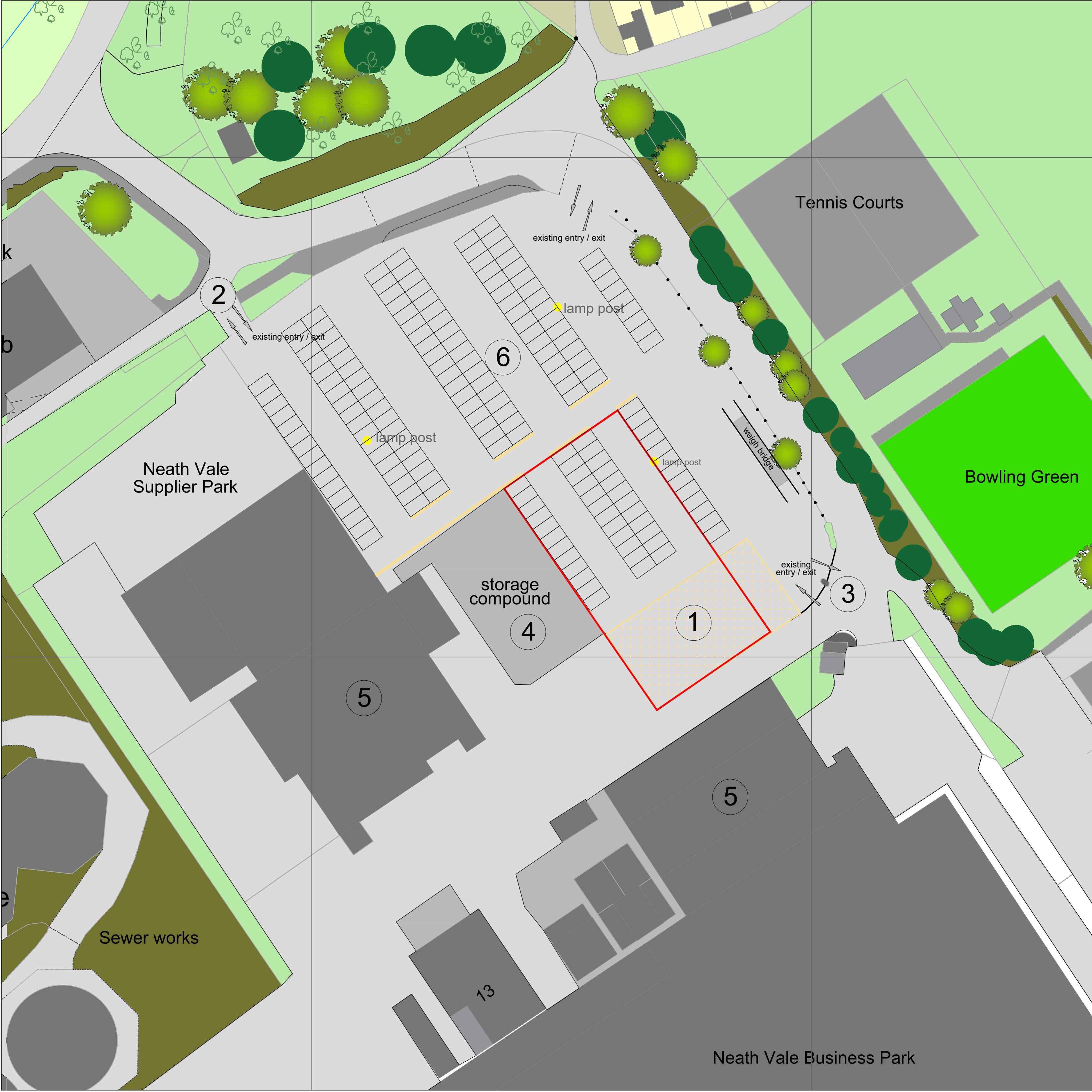
EXISTING SITE LOCATION PLAN SCALE: 1:500
