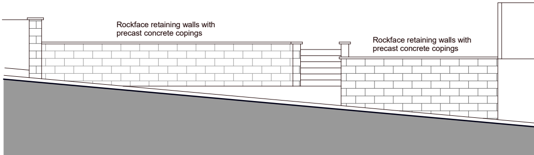
Proposed Elevation to Gardeners Lane
