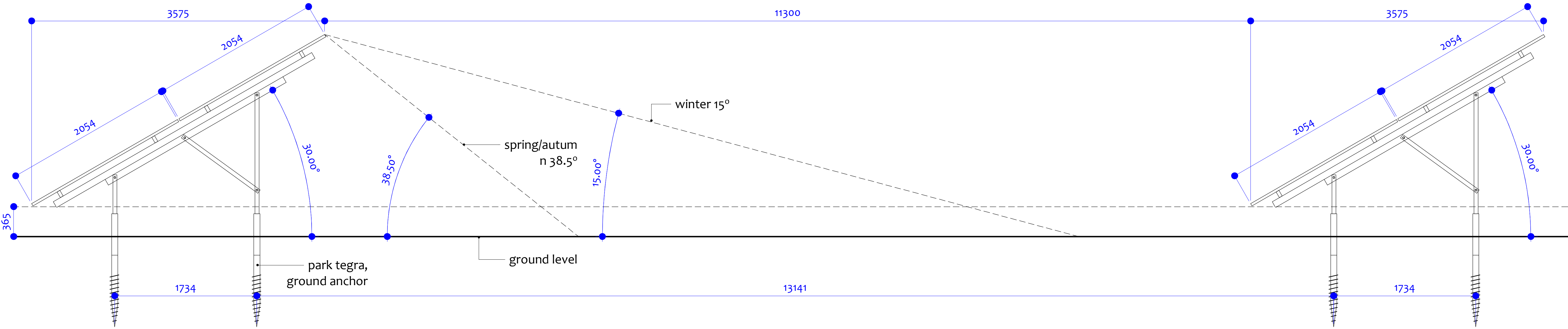
02 ARRAY SPACING (PROPOSED SITE ARRAY)
