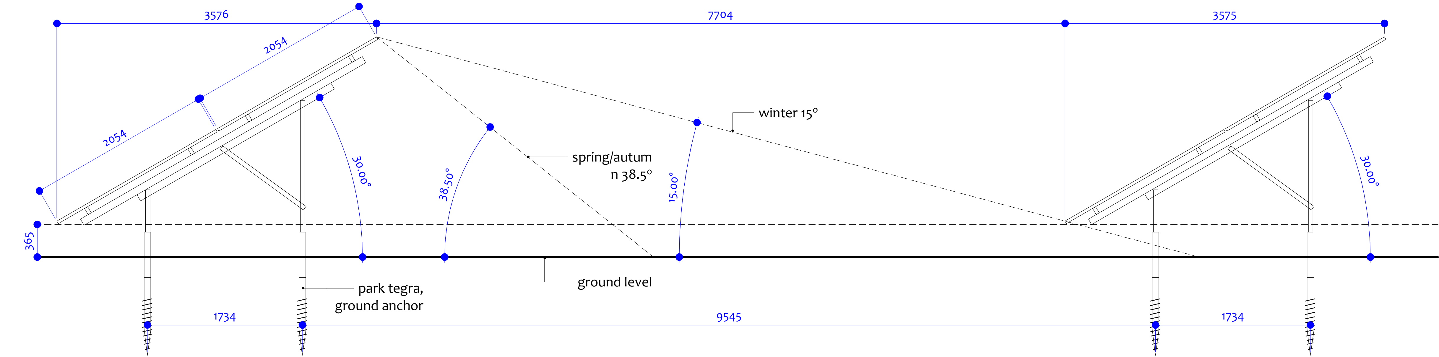
01 ARRAY SPACING (MINIMUM ARRAY TO AVOID SHADING)
