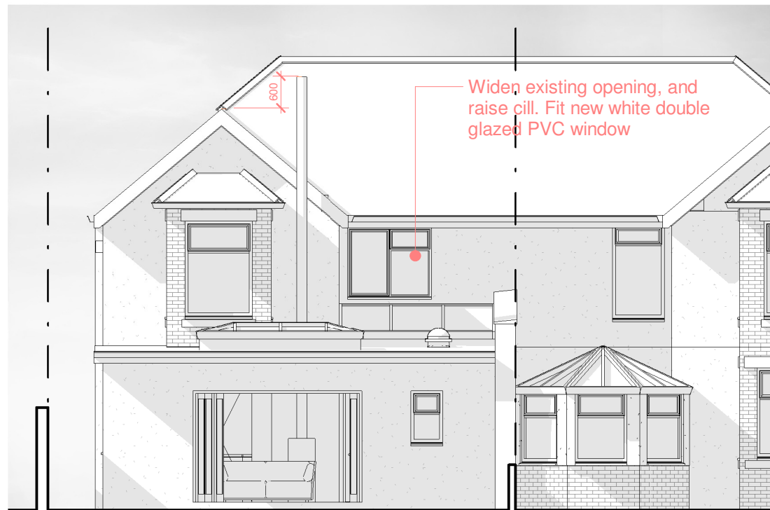
REAR - PROPOSED
