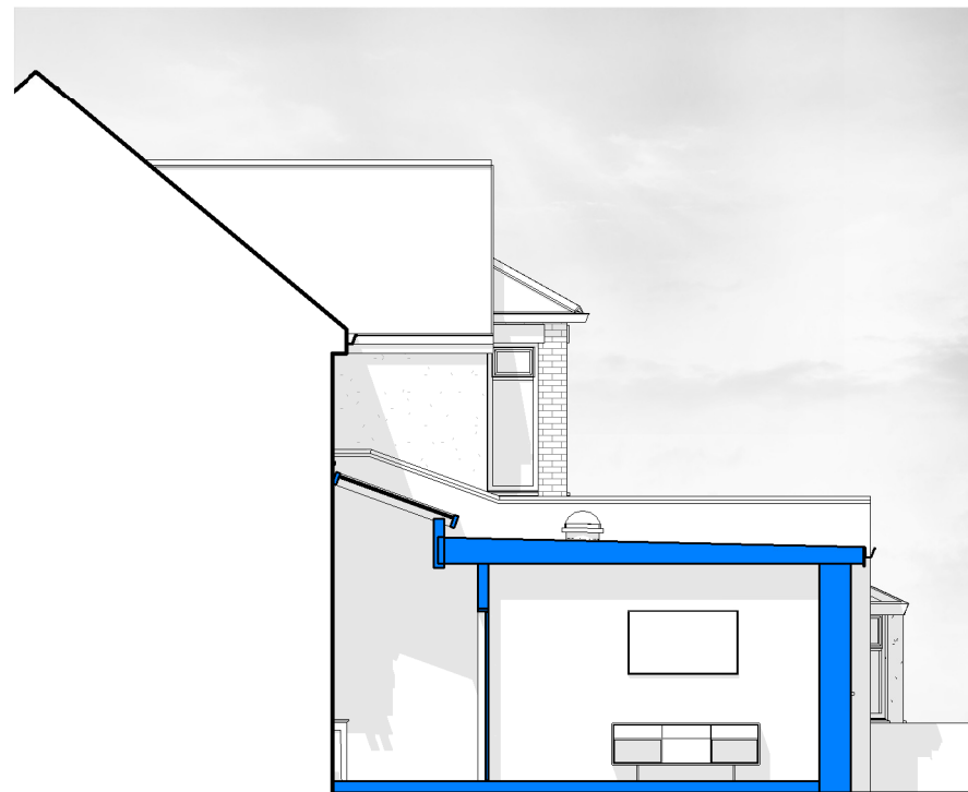
RIGHT - PROPOSED SECTION
