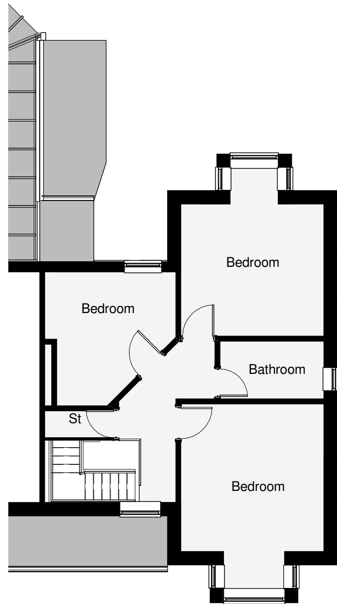
FIRST FLOOR - EXISTING 1 : 100
