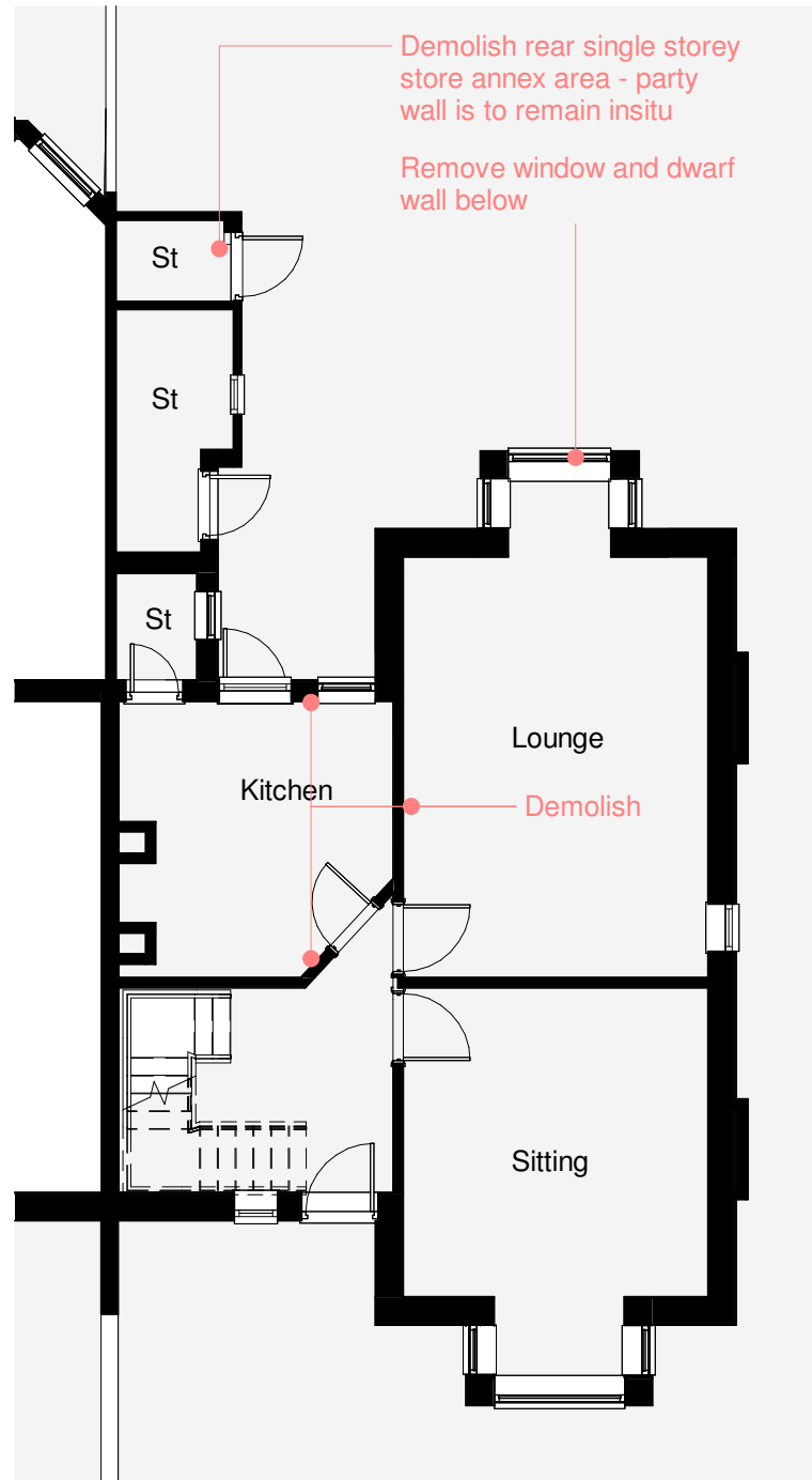
GROUND FLOOR - EXISTING 1 : 100
