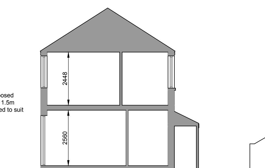
EXISTING SECTION A-A SCALE 1:100
