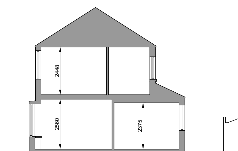
EXISTINGSECTION B-B SCALE 1:100
