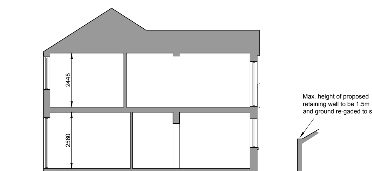
PROPOSED SECTION C-C SCALE 1:100
