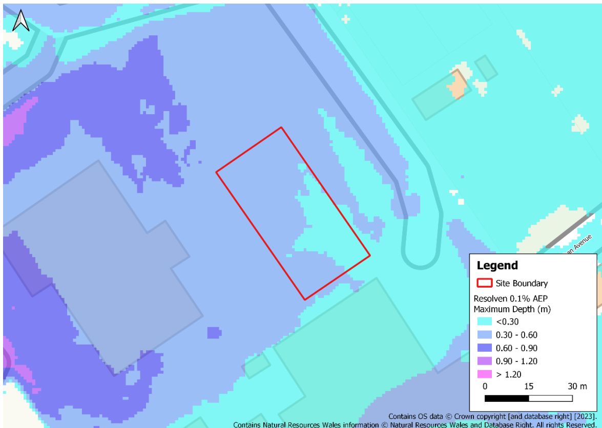
Figure 5-6 0.1% AEP maximum flood depth at site
