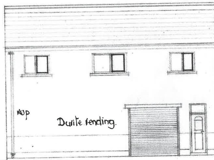
Front Elevation
