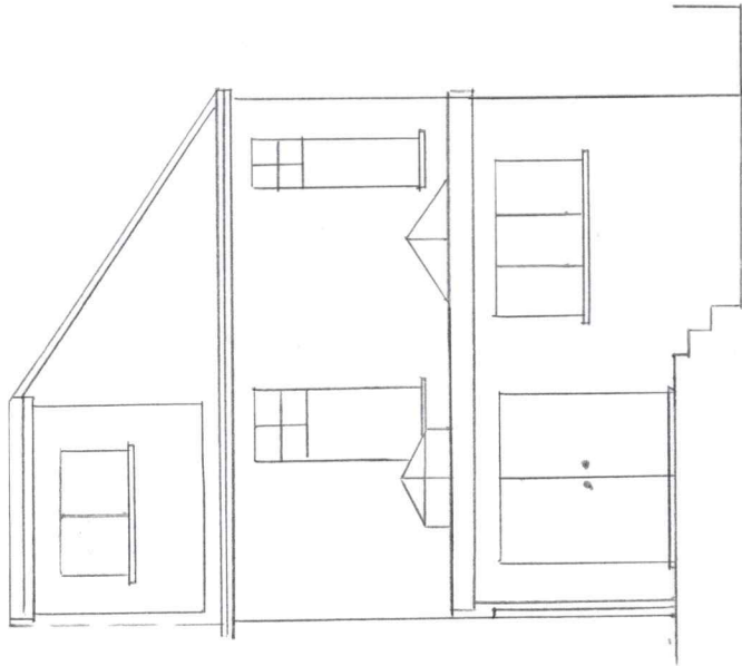
REAR ELEVATION
