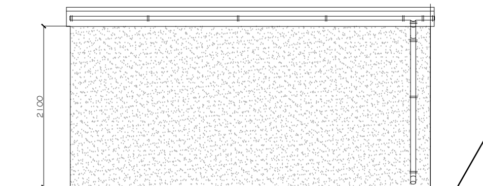
REAR ELEVATION 1 : 50
