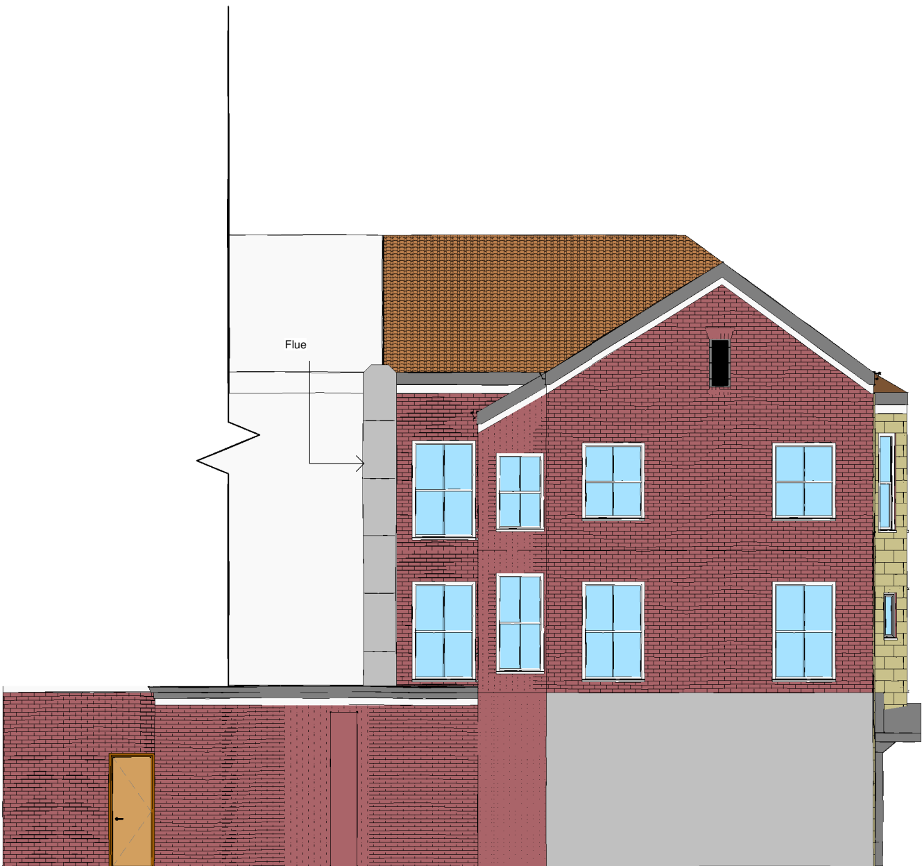
Proposed Side Elevation 2 1 : 100
