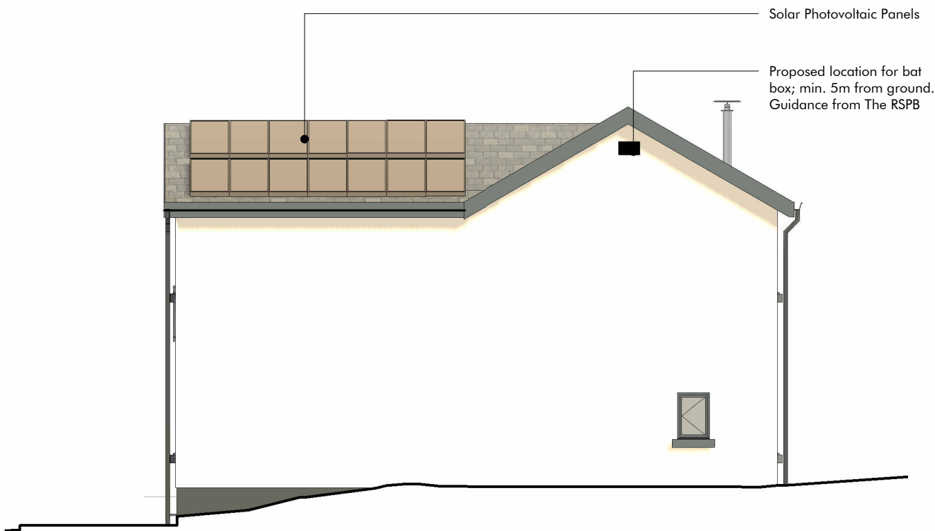
Side Elevation
