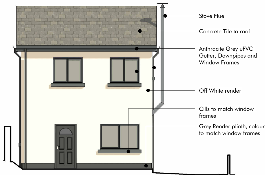
Front Elevation
