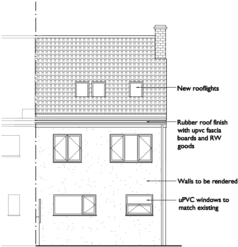
South-West Facing Elevation
