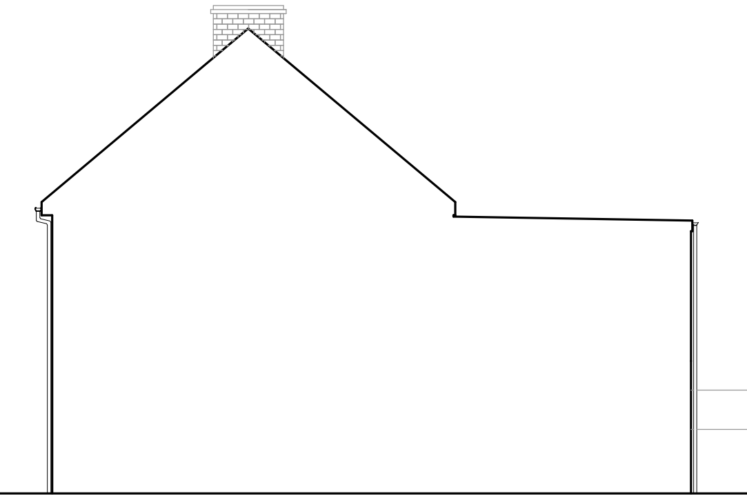
North-East Facing Elevation
