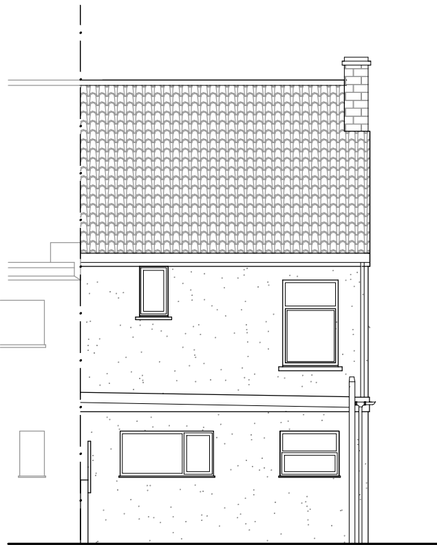
South-West Facing Elevation
