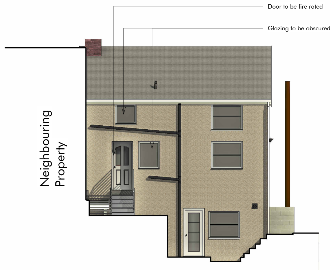
Rear Elevation
