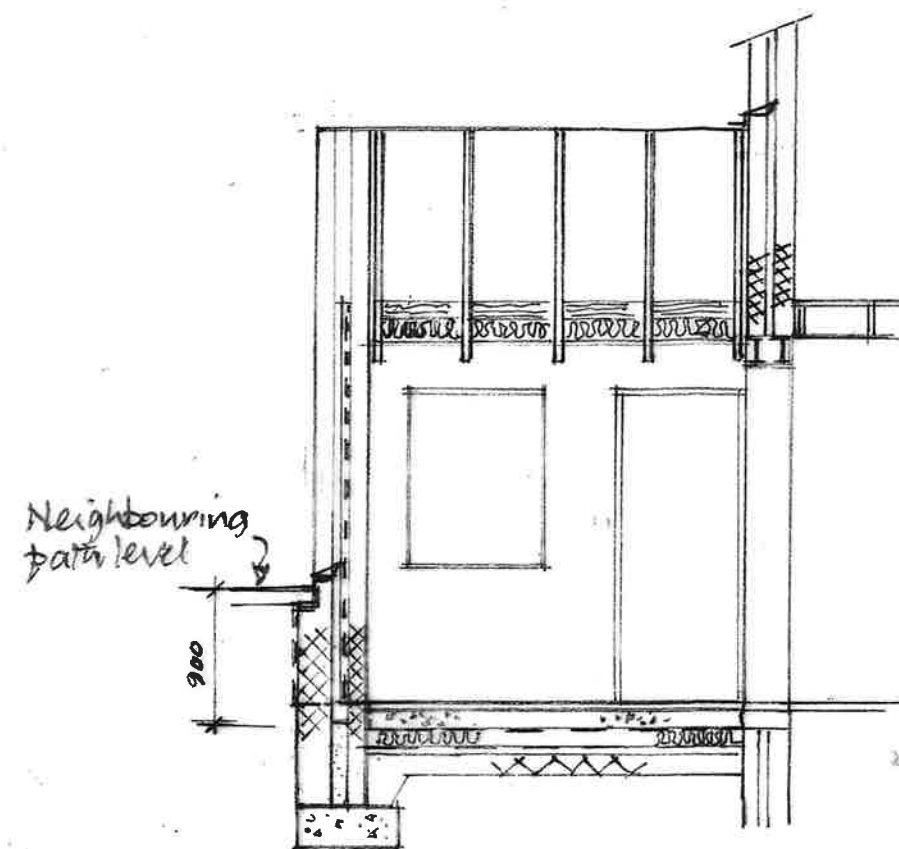
Section B-B
