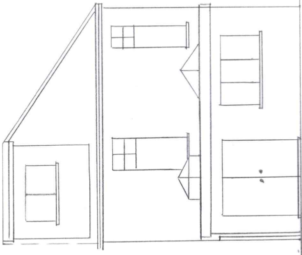
REAR ELEVATION
