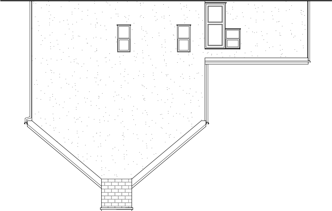
South-East Facing Elevation
