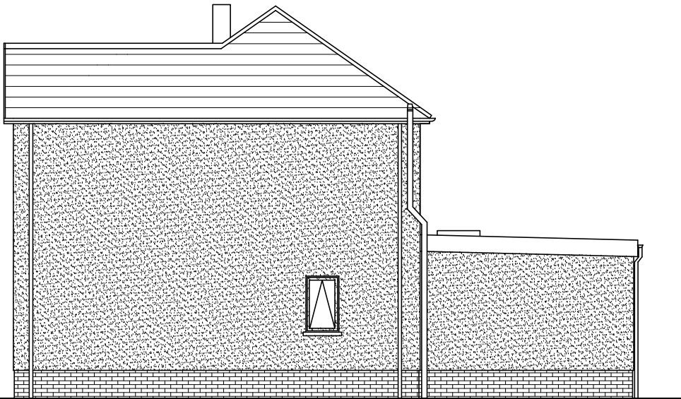
Existing Side Elevation (as existing)
