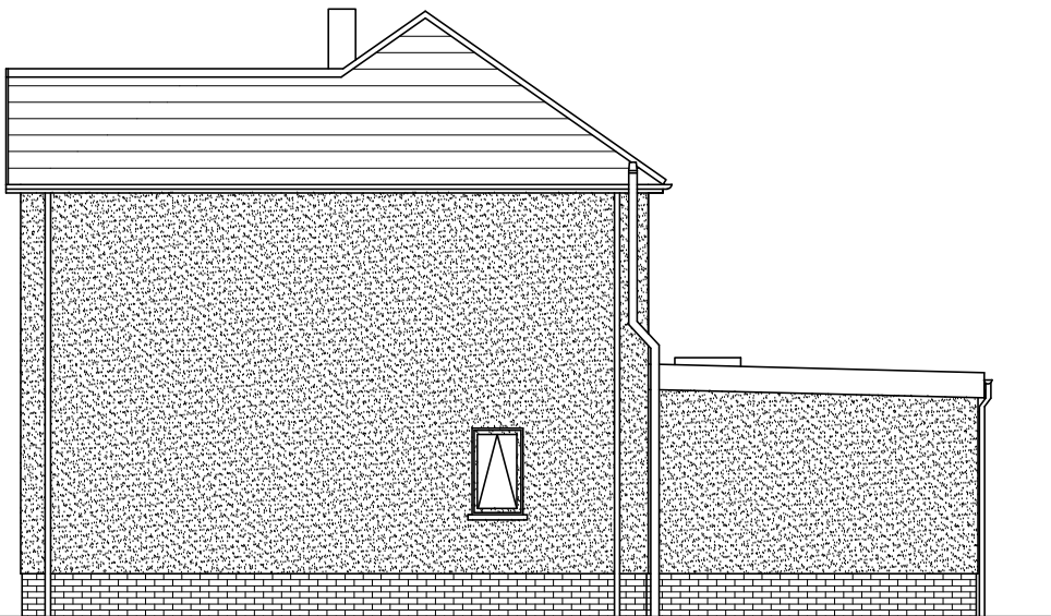
Proposed Side Elevation (as existing)
