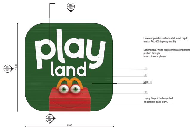
01 Play Logo 1100mm: Front Elevation 1:10
