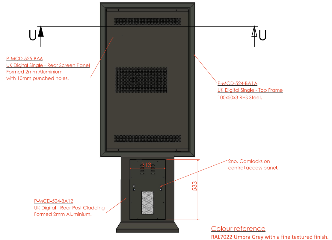
Rear View
