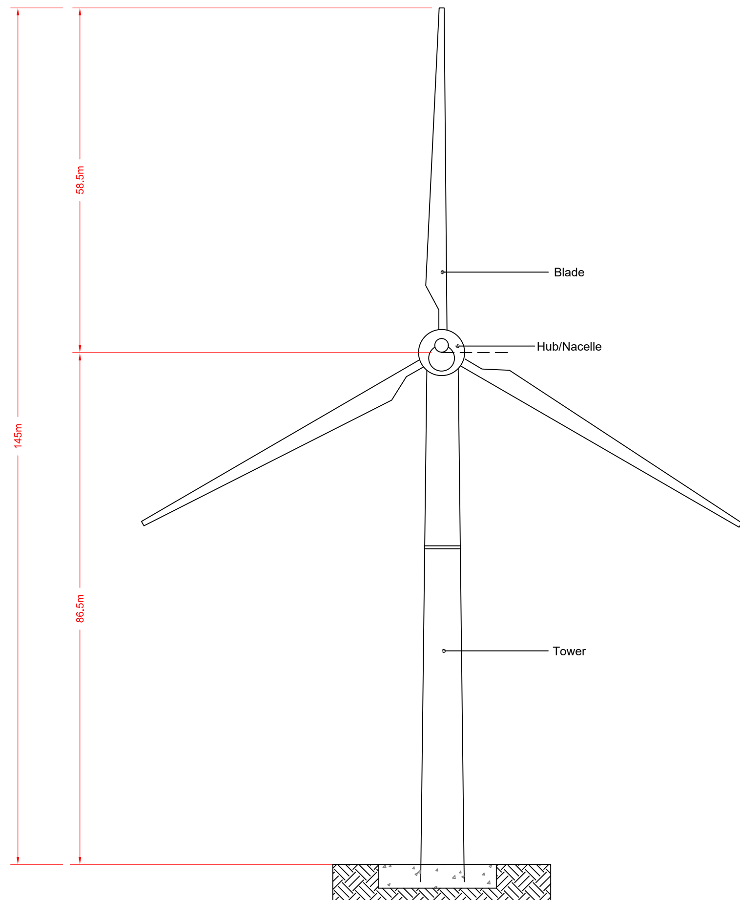
Figure B2 Wind turbine elevations - 58.5m blade length (117m rotor diameter)
