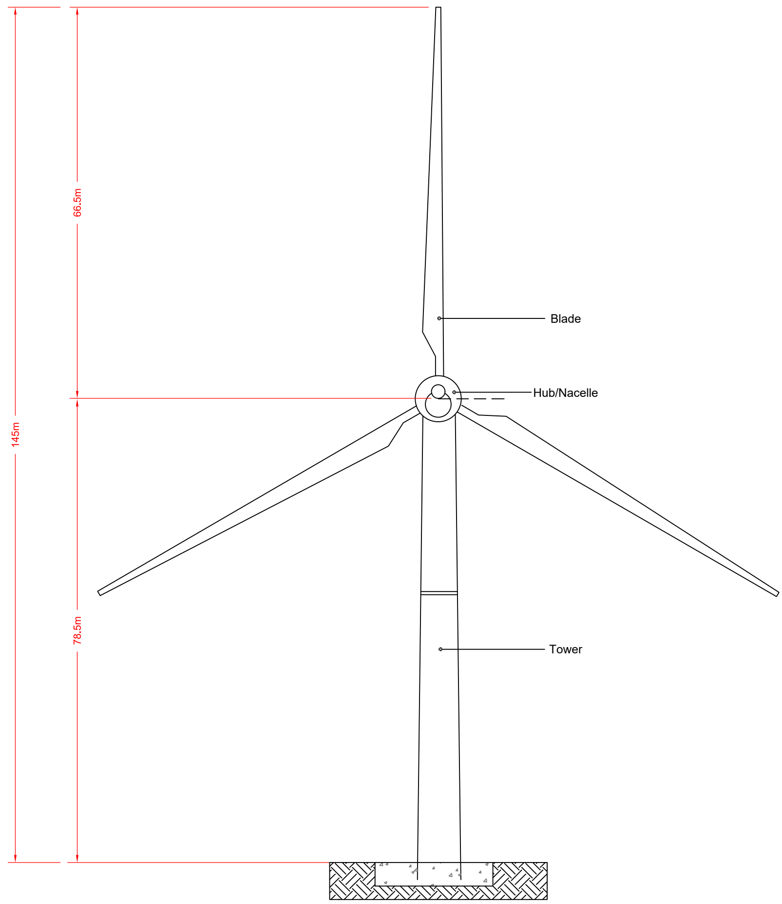
Figure B1 Wind turbine elevations - 66.5m blade length (133m rotor diameter)
