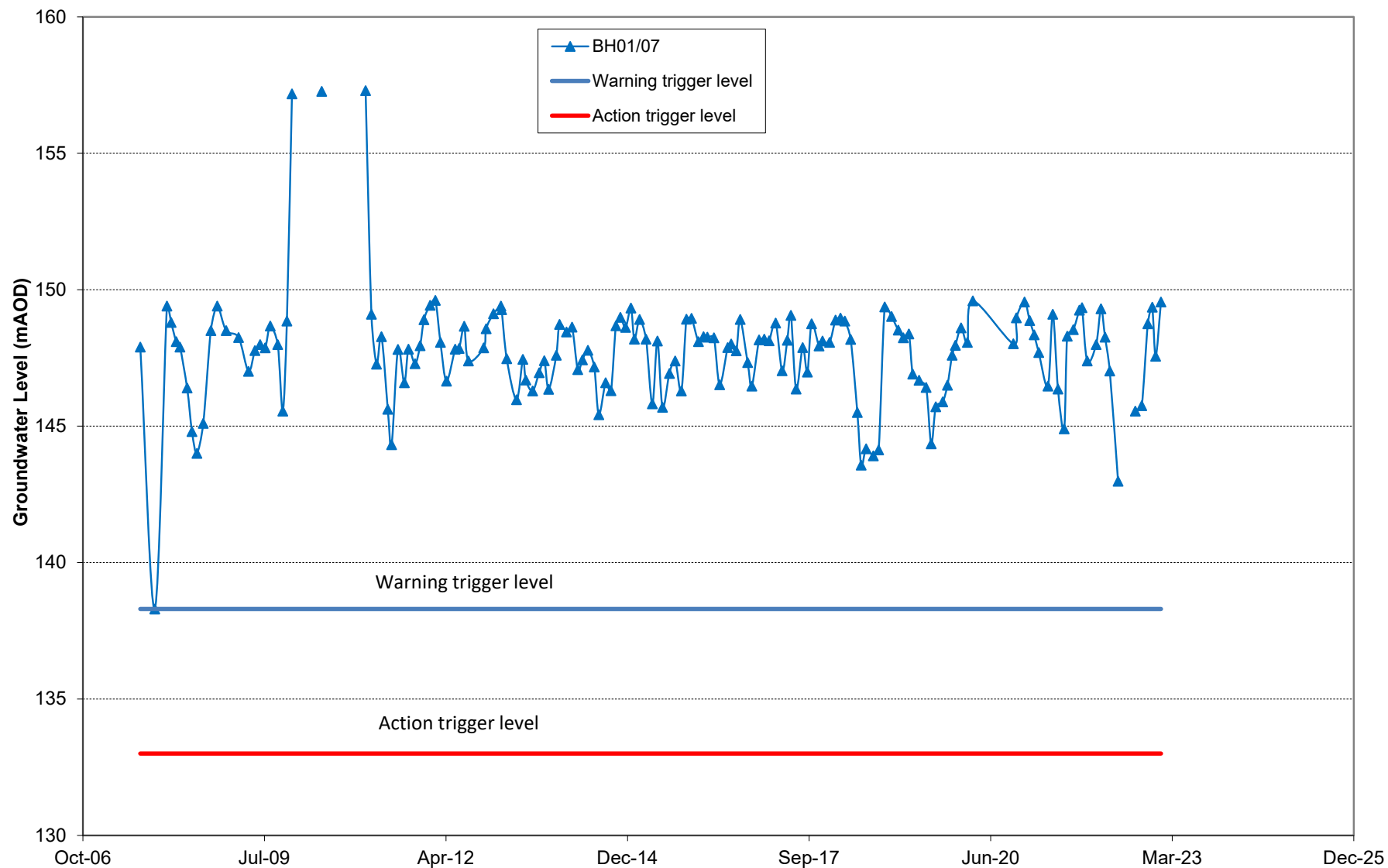
GILFACH QUARRY - BH01/07 HYDROGRAPH AND TRIGGER LEVELS
