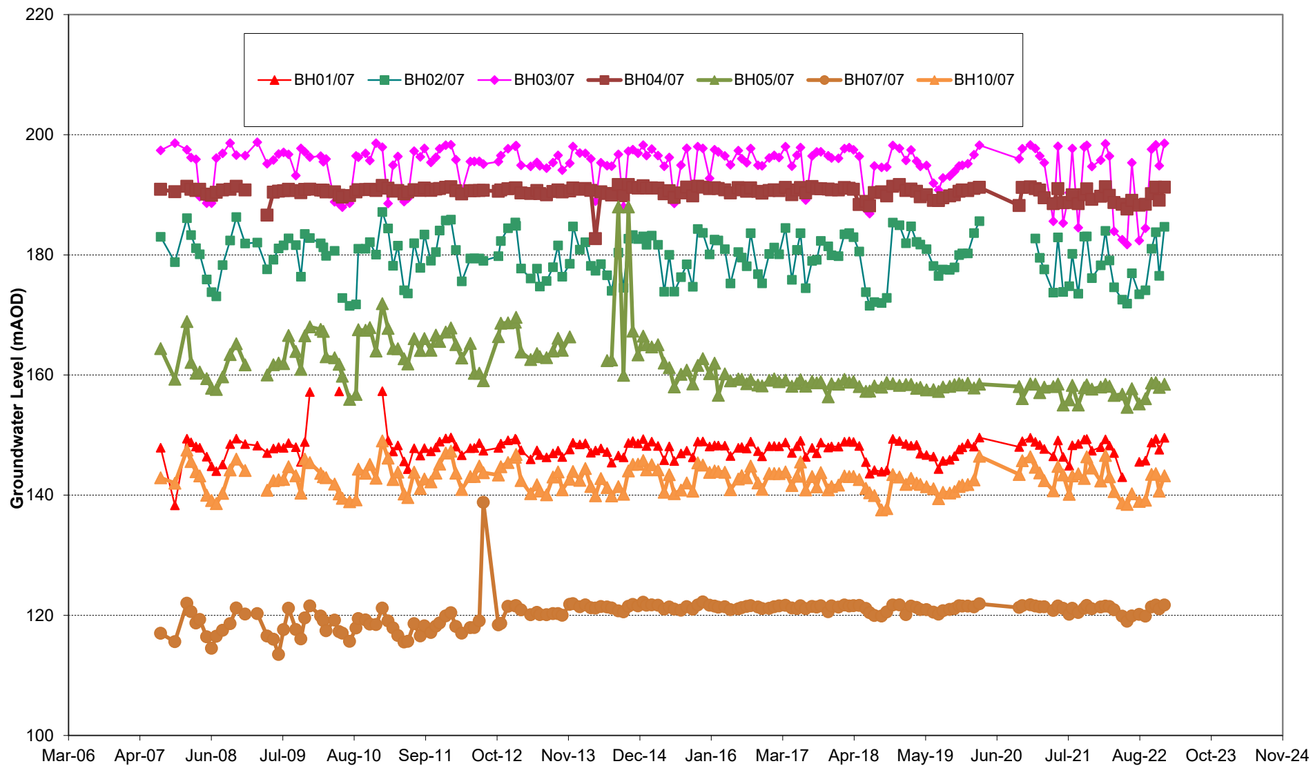
GILFACH QUARRY - COMPOSITE LONG TERM GROUNDWATER HYDROGRAPH
