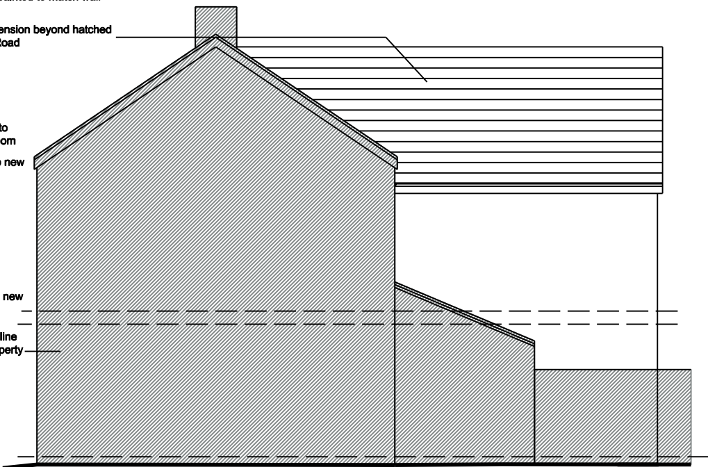
Proposed Left Side Elevation (From No. 1 Gynol Road)
