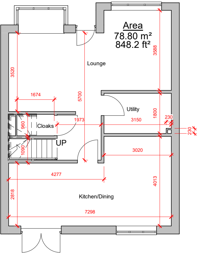
G Ground Floor 1 : 100
