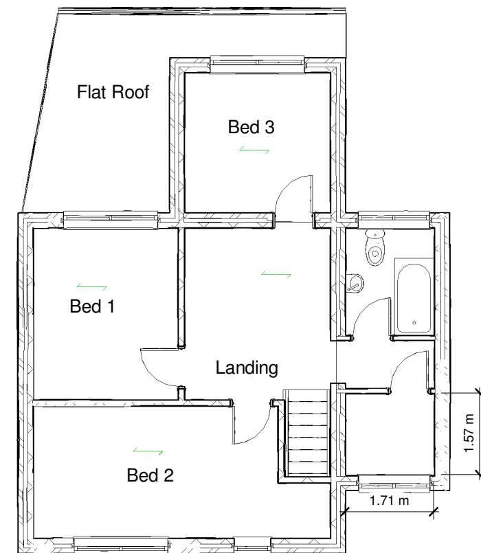
Proposed FF 1 : 100
