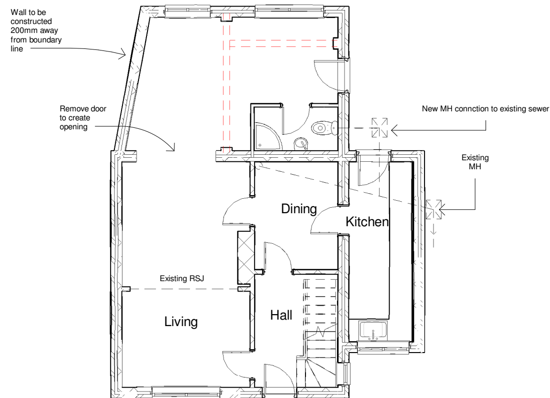
Proposed GF 1 : 100
