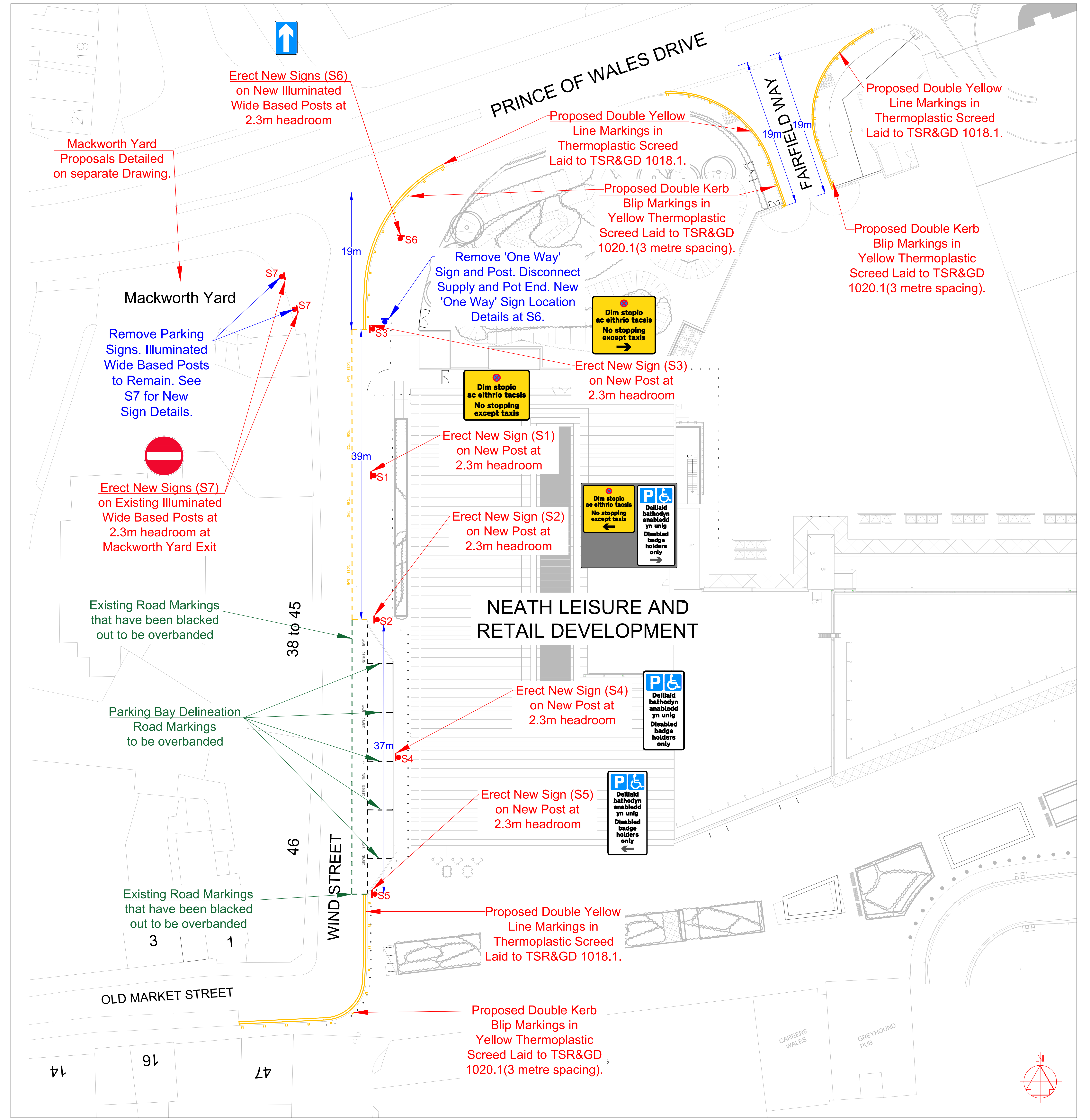
PROPOSED TRAFFIC REGULATION ORDER LAYOUT PLAN - SCALE 1:200
