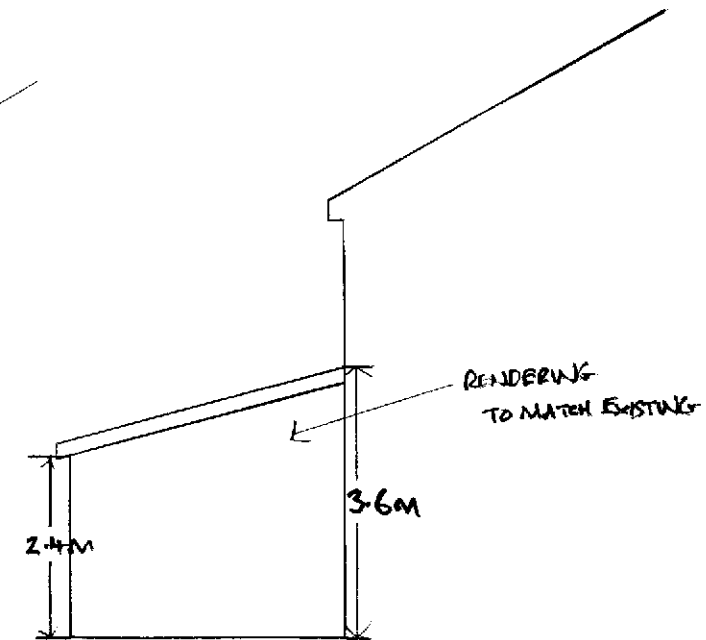
SIDE ELEVATION TO NEIGHBOUR PROPOSED
