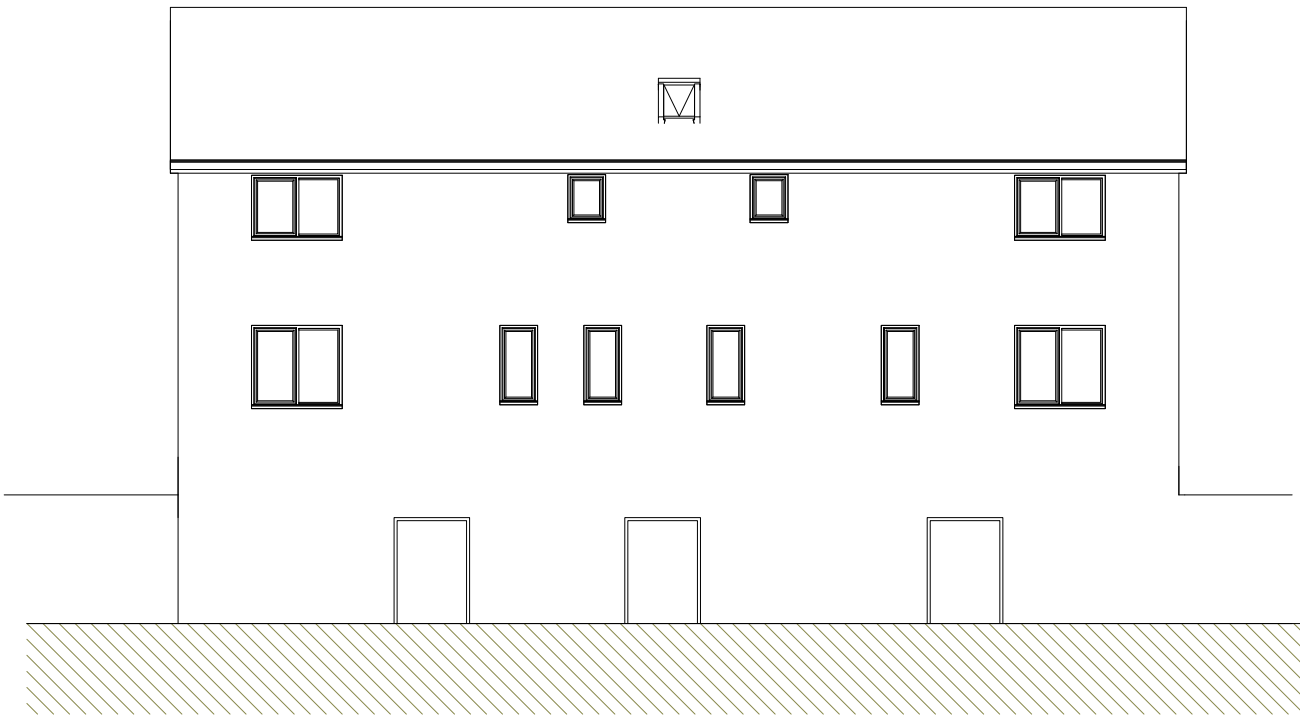
3 South West 1 : 100
