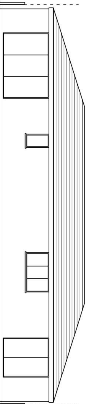
Garden Elevation
