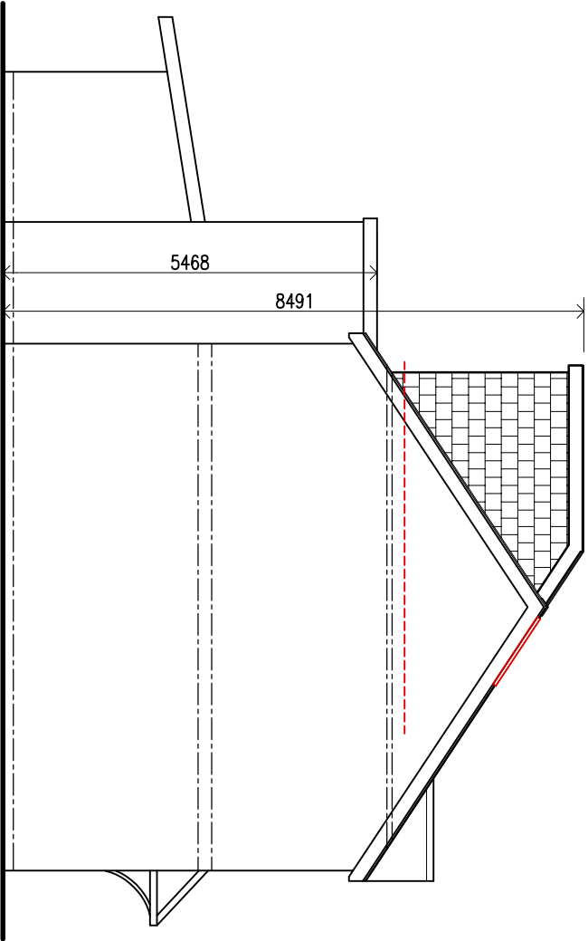
PROPOSED SIDE SECTIONAL ELEVATION. (1:100)
