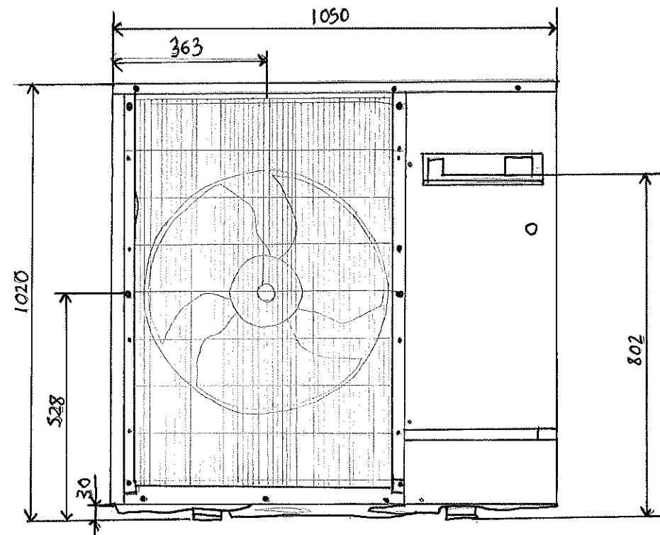
FRONT VIEW
