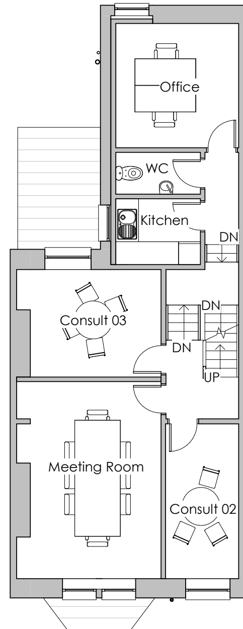
2 First Floor 1 : 100
