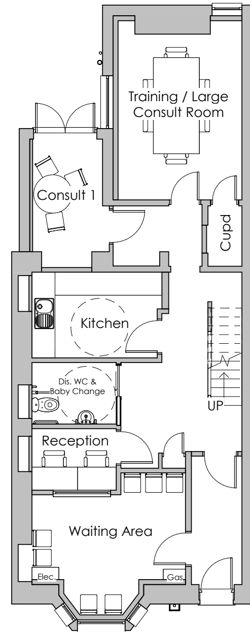
1 Ground Floor 1 : 100
