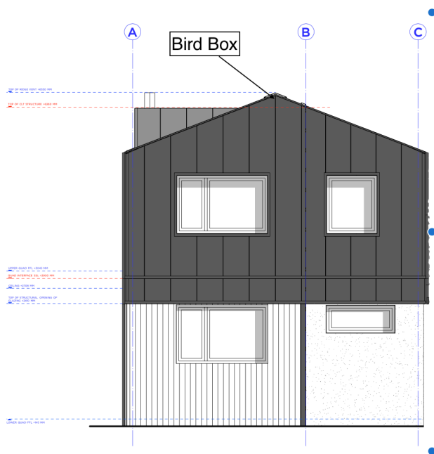
FRONT ELEVATION | 1:25
