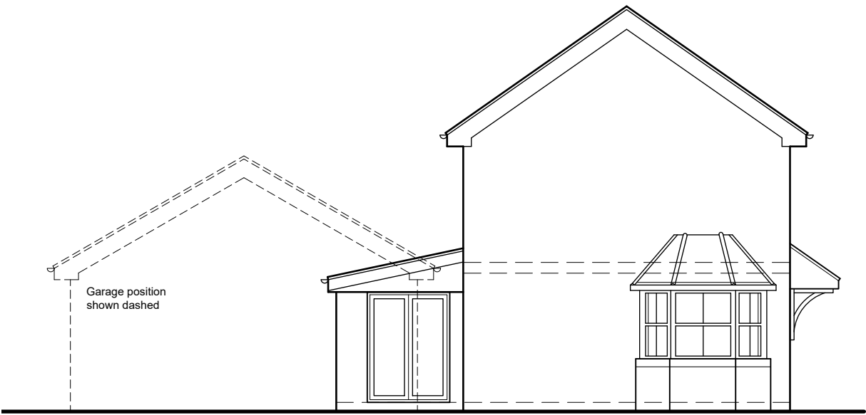
Side Elevation
