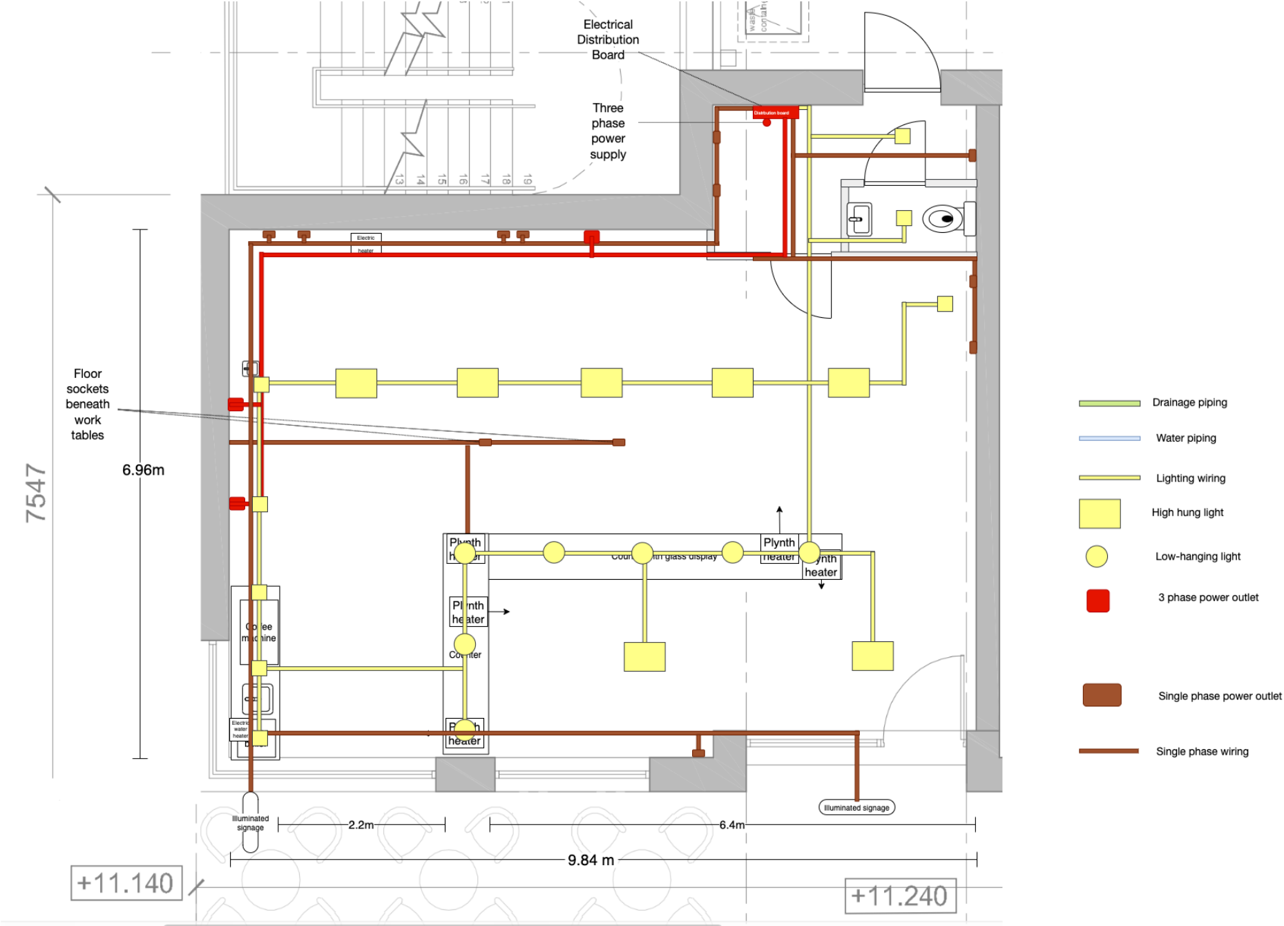
Floor Plan with electrical only
