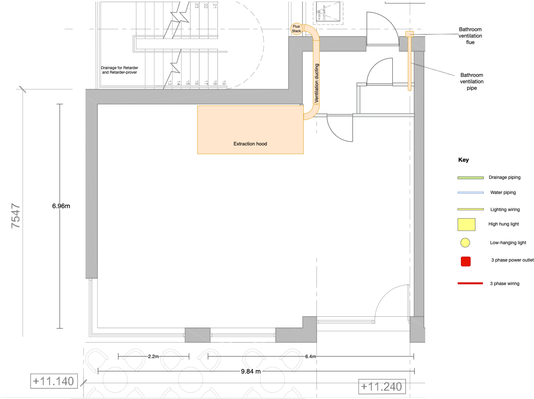
Floor Plan with ventilation only
