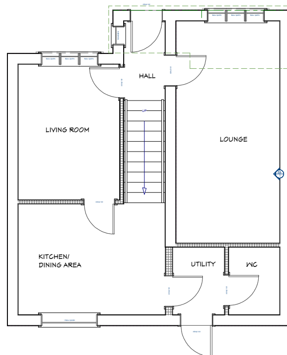
GROUND FLOOR PROPOSED
