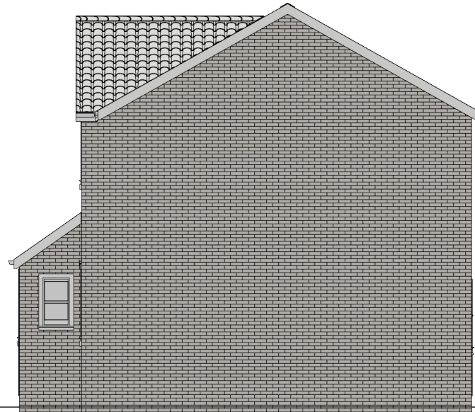
SIDE ELEVATION PROPOSED
