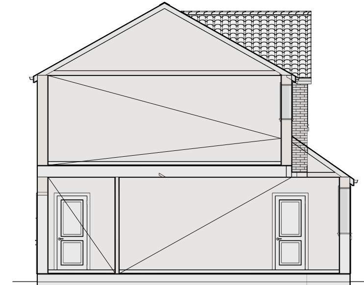
SECOND SIDE ELEAVTION (SECTION THROUGH) PROPOSED
