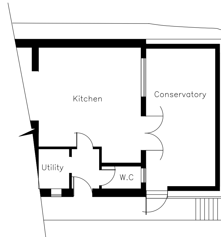
Proposed Floorplan 1:100
